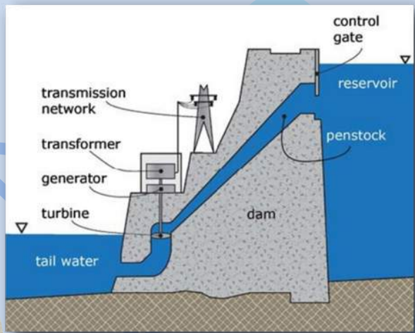
The Bachelor third year students studying the schematic of reservoir-based hydropower system (PHY701 unit).
